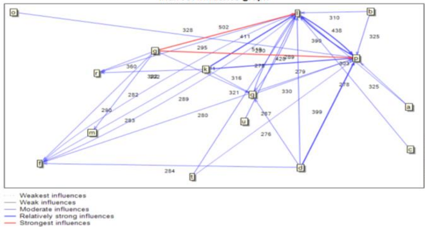
Indirect influence graph
